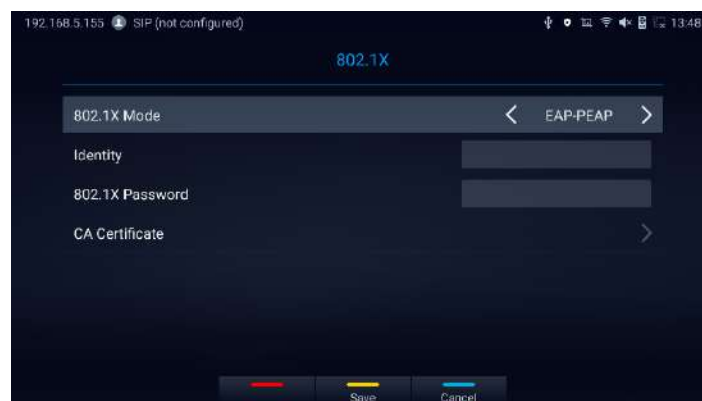
Figure 32: 802.1X - EAP-PEAP
