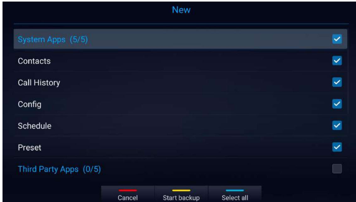
Figure 132: New Backup
