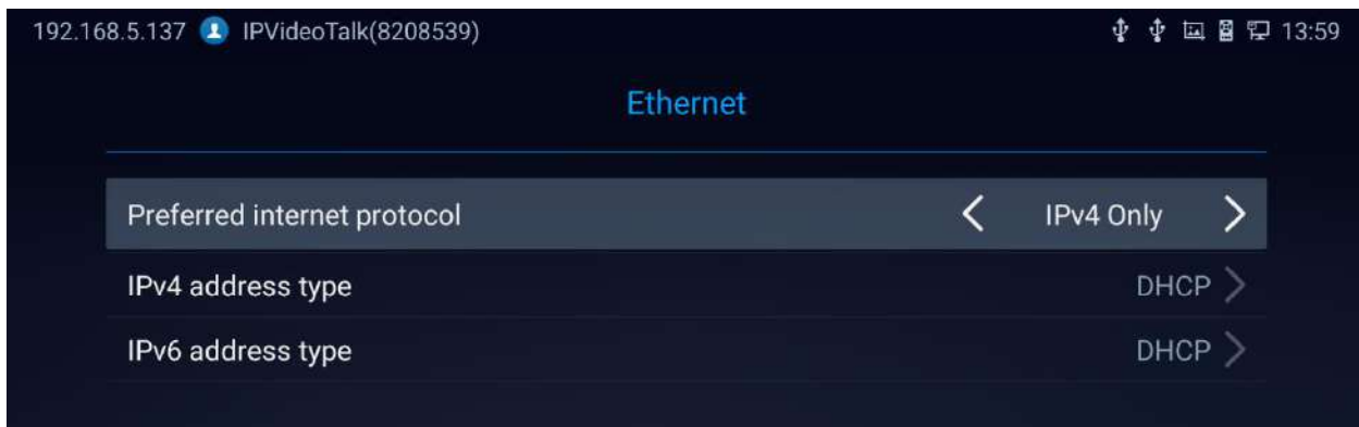
Figure 18: Ethernet Settings
