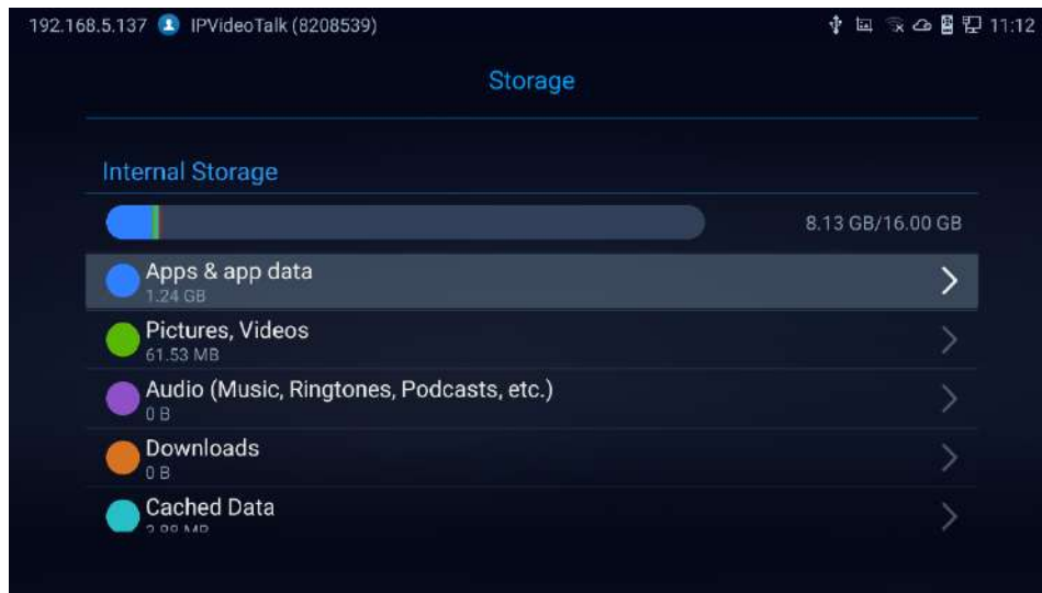
Figure 15: System Storage
