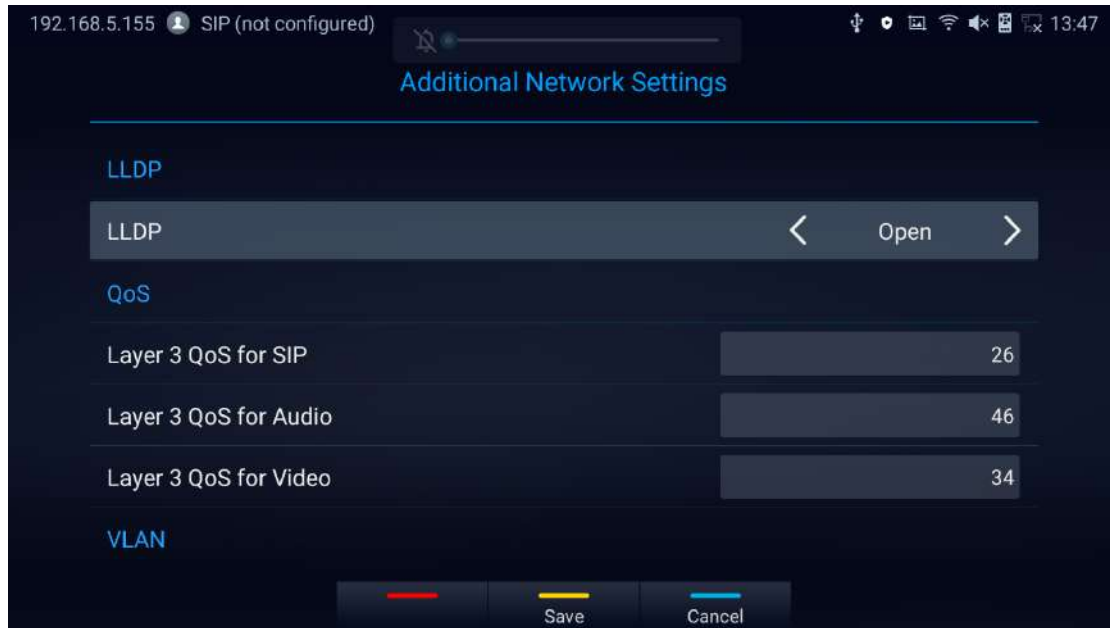
Figure 28: LLDP/VLAN Settings
