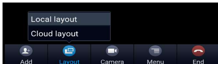
Figure 60: Layout customization
