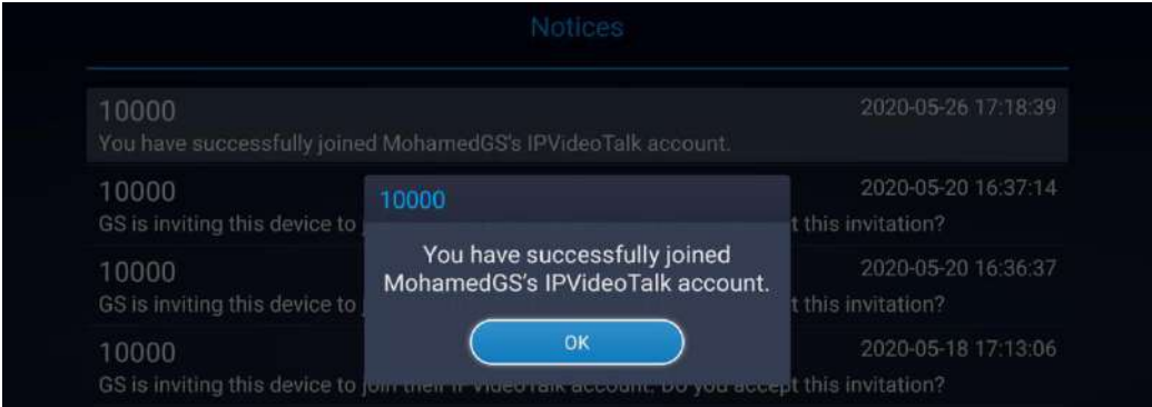
Figure 148: Notices - Details
