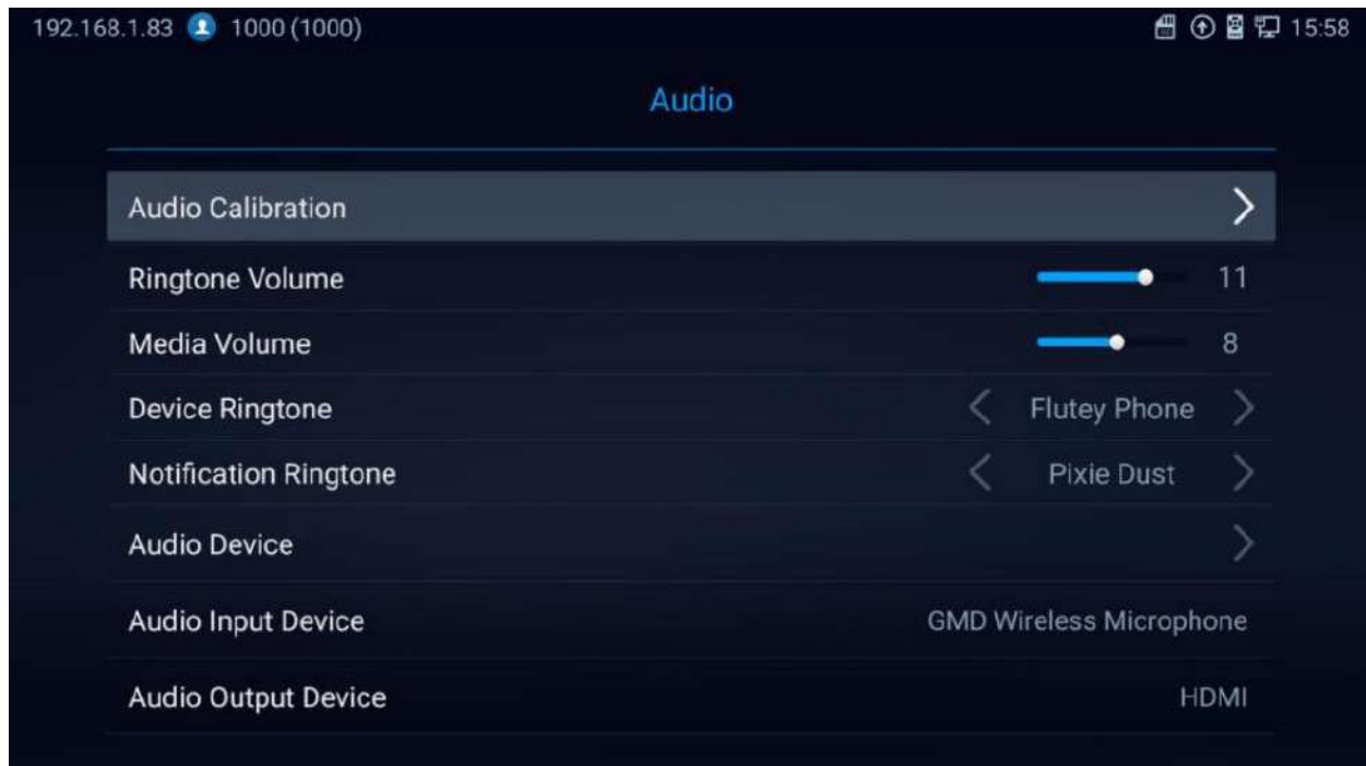
Figure 40: Audio Calibration
