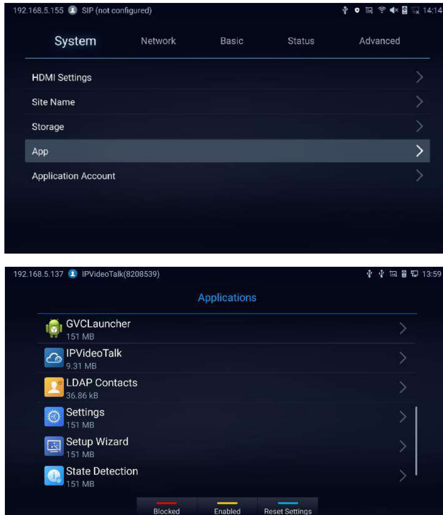
Figure 139: System - Apps
