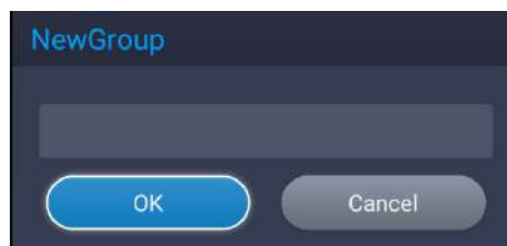
Figure 50: New Group
