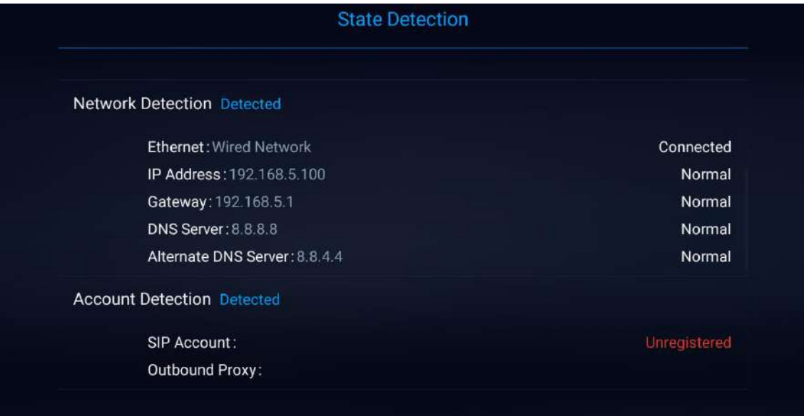
Figure 137: Network/Account Detection
