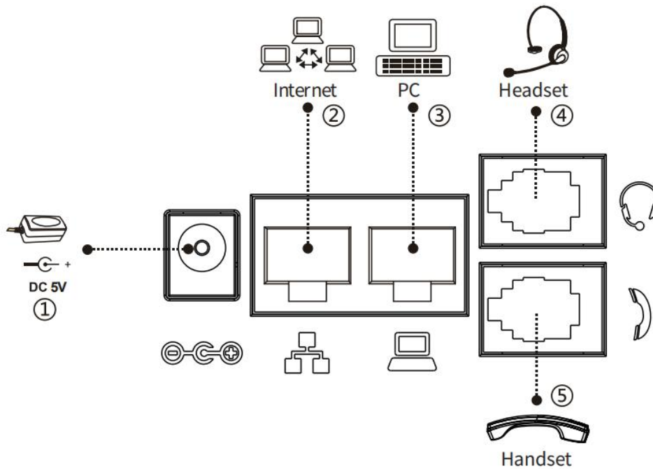
Picture 3 - Connecting to the Device
