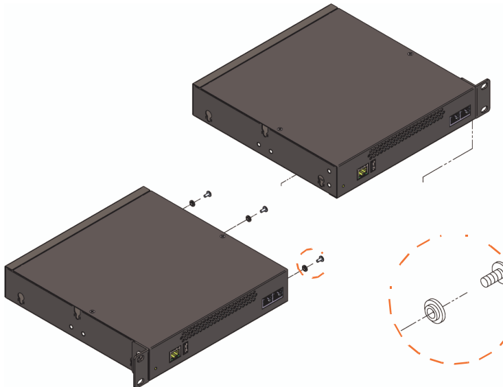
Figure 7: Side-by-side Rack Mounting
